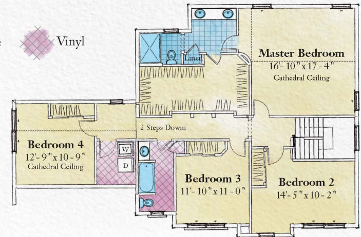
Second Floor Plan Optional Bedroom 4
