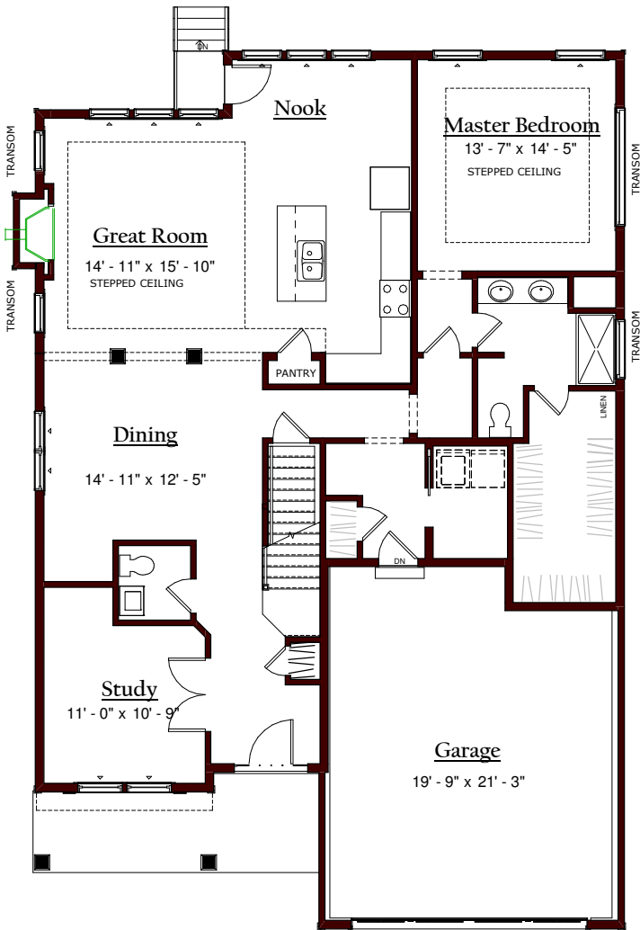
FIRST FLOOR PLAN - artwork
