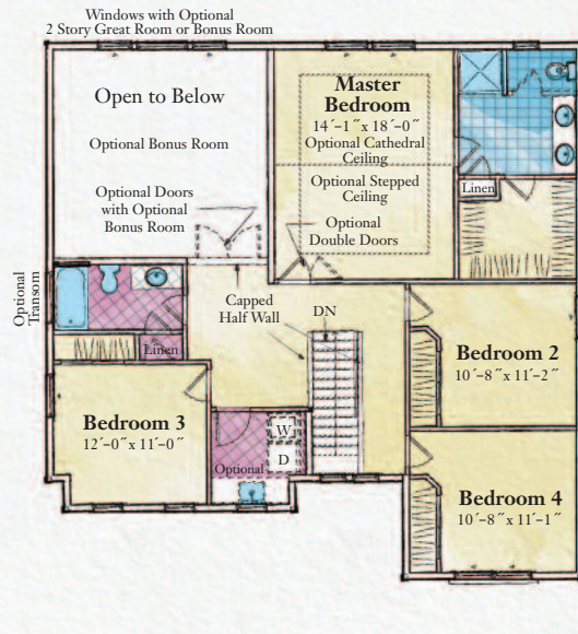
Second Floor Plan Elevation A
