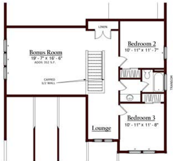
SECOND FLOOR PLAN - artwork bonus room
