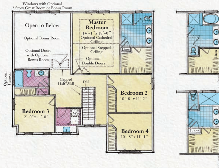
Second Floor Plan Elevation A
