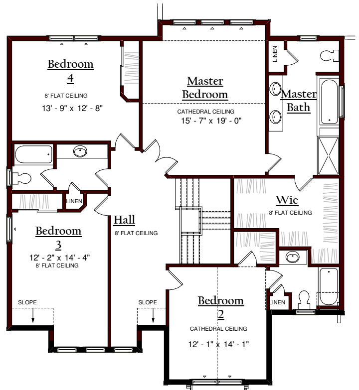
SECOND FLOOR
